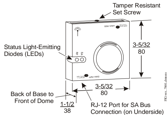
WRZ-7860-0 Receiver Dimensions and Physical Features, in./mm
